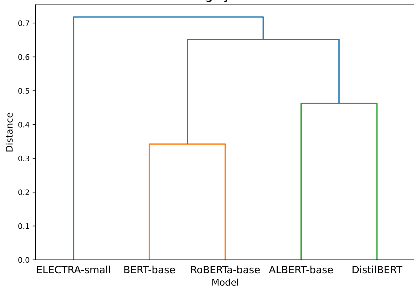
Model Clustering by Noise Robustness
