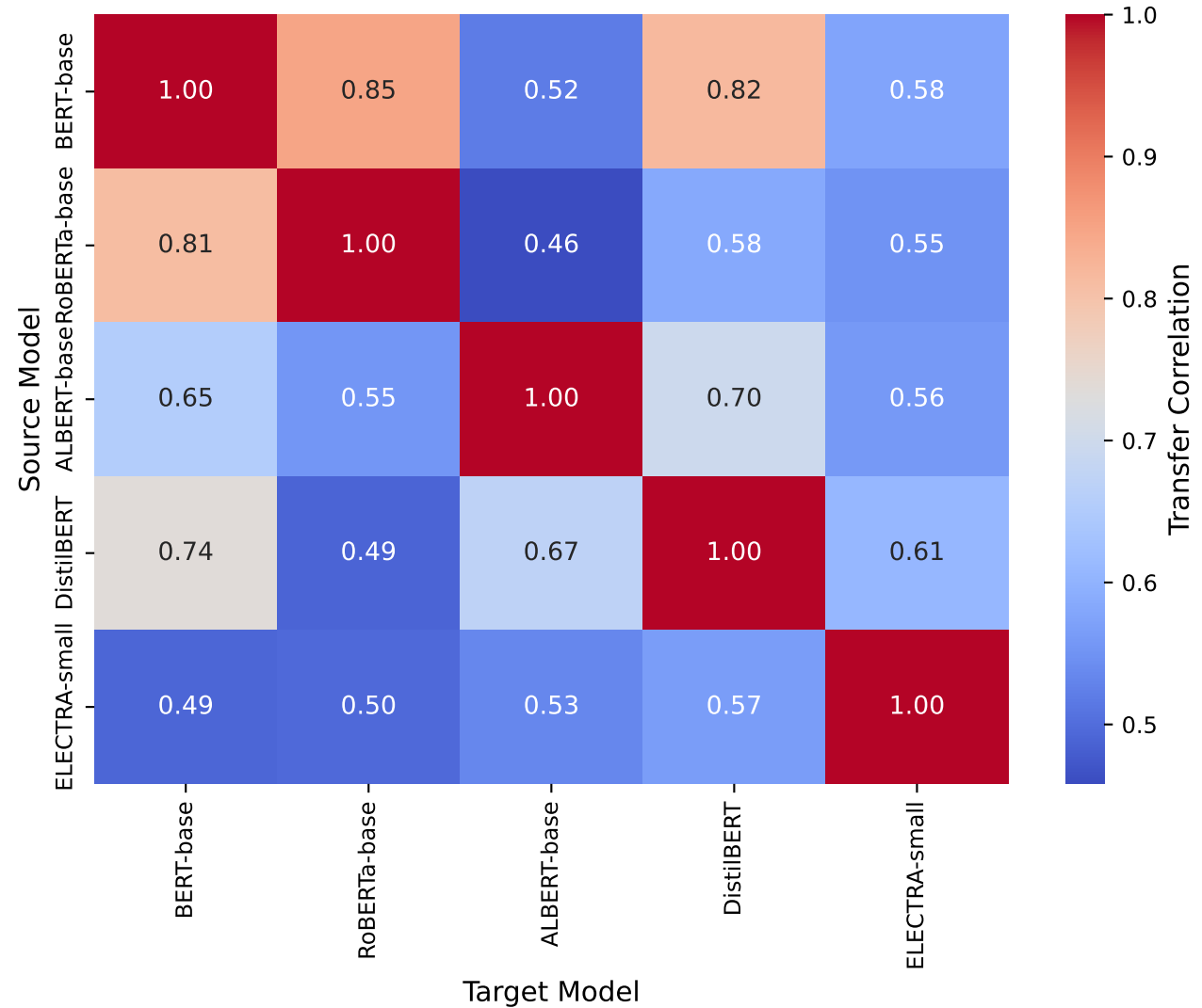
Cross-Model Noise Pattern Transfer
